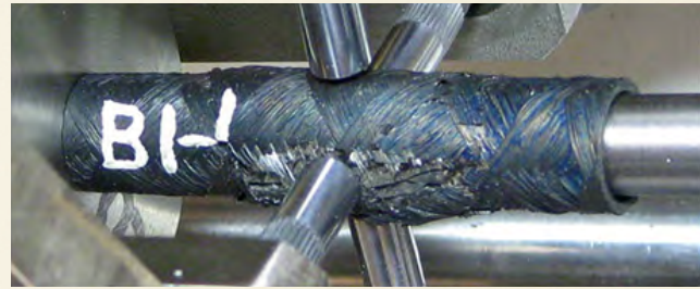
Figure 2. (top) Round 6 triplex tube undergoing mandrel-driven expanding plug burst testing.
