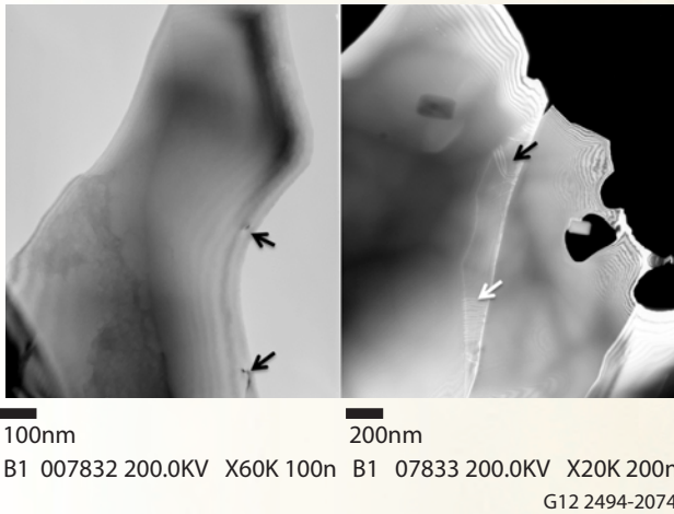
Figure 2. TEM micrographs of Ti_3SiC_2 irradiated with a Cf neutron source to a dose of \sim 10^{-7} dpa. As expected, such a low dose resulted in no visible irradiation damage. Dislocations (black arrows) and stacking faults (white arrow) can be seen in both the a) bright-field and b) dark-field images of different regions.
