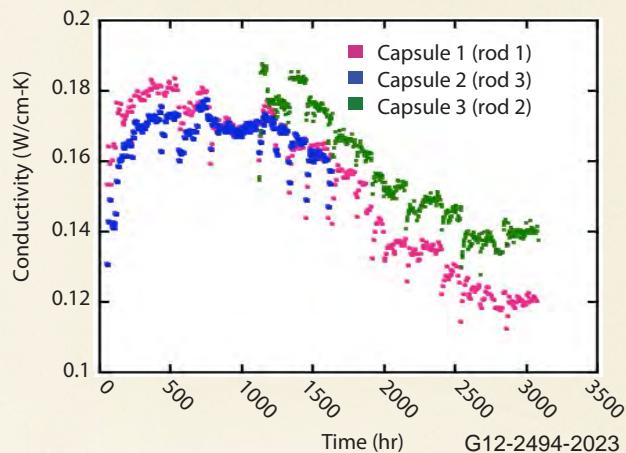
Figure 3. Thermal conductivity variation with irradiation exposure for thermal power greater than 4 MW.
