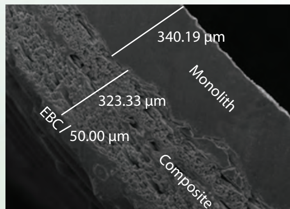
Figure 1. SEM micrograph cross section showing the three layers of the triplex cladding design.
