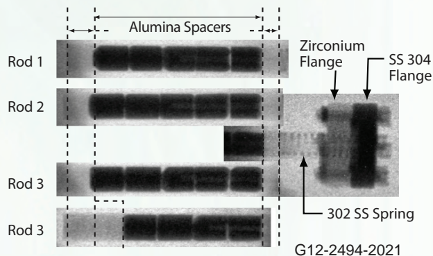
Figure 1. Neutron radiographs of four liquid metal gap filled fuel rod assemblies.
