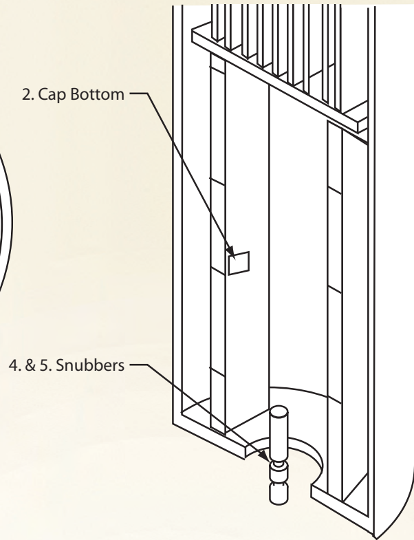
Figure 3. Artist's rendition of a cutaway of the bottom of the UNLV ICSBEP cassette showing the snubber (keeps the cassette centered in the ATRC flux trap) and the bottom support for the aluminum bars.
