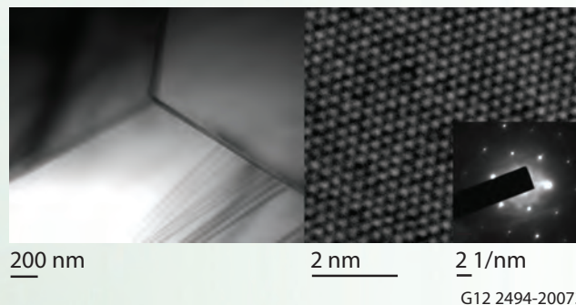
Figure 1. TEM micrographs of unirradiated Ti_3AlC_2 showing: a) a low-resolution, bright-field image of a triple point, b) a high-resolution image near the edge of the bottom grain in Figure 1(a). The inset shows a selected-area diffraction pattern from the same region with hexagonal symmetry of the basal planes.
