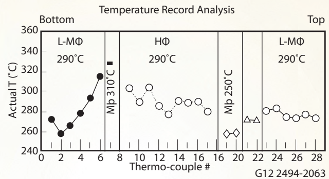
Figure 3. Actual temperature deviations from the calculated set points showing excellent overall thermal performance.
