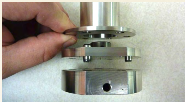
Figure 2. Side view of the shear punch fixture. G12 2494-2057
