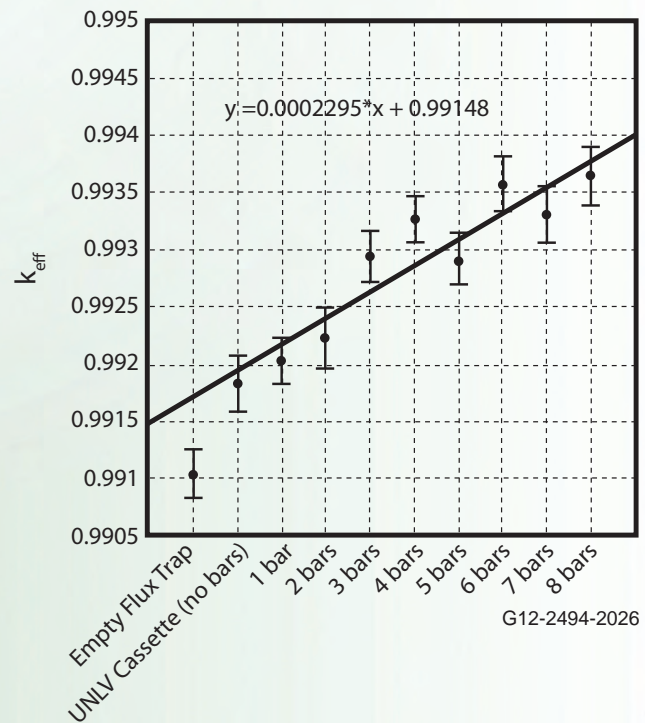
Figure 1. Effect of the Aluminum Bars in the UNLV ATRC Cassette on Reactor Criticality. The initial experiment will include all eight bars. They will then be removed one at a time, starting in the center. Thus, having seven bars does not mean one of the two outermost bars will be removed.
