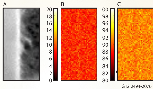
Figure 3. Annular dark-field image of lath boundary in as-received model steel, B) weight percent chromium map (bulk concentration: ~8.68% Cr), C) weight percent iron map.
