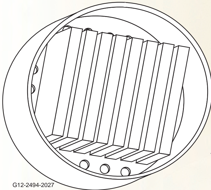
Figure 2. Artist's rendition of a cutaway of the UNLV ICSBEP cassette showing the water holes and the bars penetrating the spacer.
