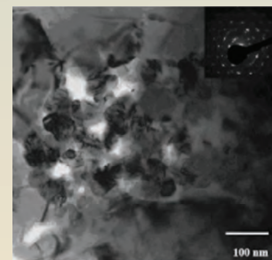
Nanocrystalline copper, following irradiation to 0.34 dpa
