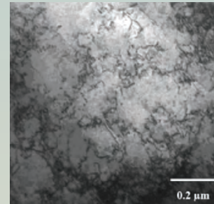
Conventional copper, after irradiation
