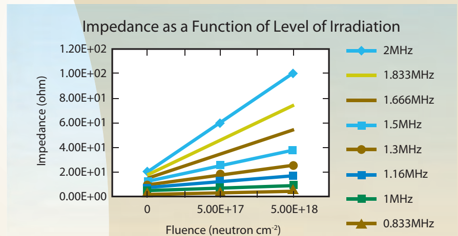
Figure 1. The preliminary results indicate a correlation between irradiation level and impedance in irradiated silicon carbide, a future reactive fuel clad material.
