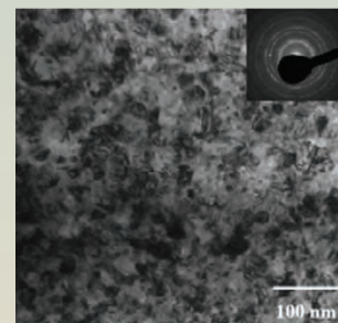
Nanocrystalline copper, before irradiation
