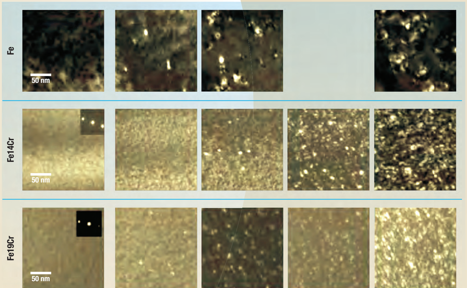
Figure 1. Dark field microscopic images show 50-nm samples of pure Fe, Fe-14Cr and Fe-19Cr single crystal material that were irradiated at the Intermediate Voltage Electron Microscope/Tandem Facility at Argonne National Laboratory. The samples were irradiated at 450°C with irradiation doses of (each row, from left): 0, 1 \times 10^{14} , 4 \times 10^{14} , 7 \times 10^{14} and 1 \times 10^{15} ion/cm 2 . Alloy samples of the same materials will be subjected to neutron irradiation at similar dosage levels in the Advanced Test Reactor and re-examined.
