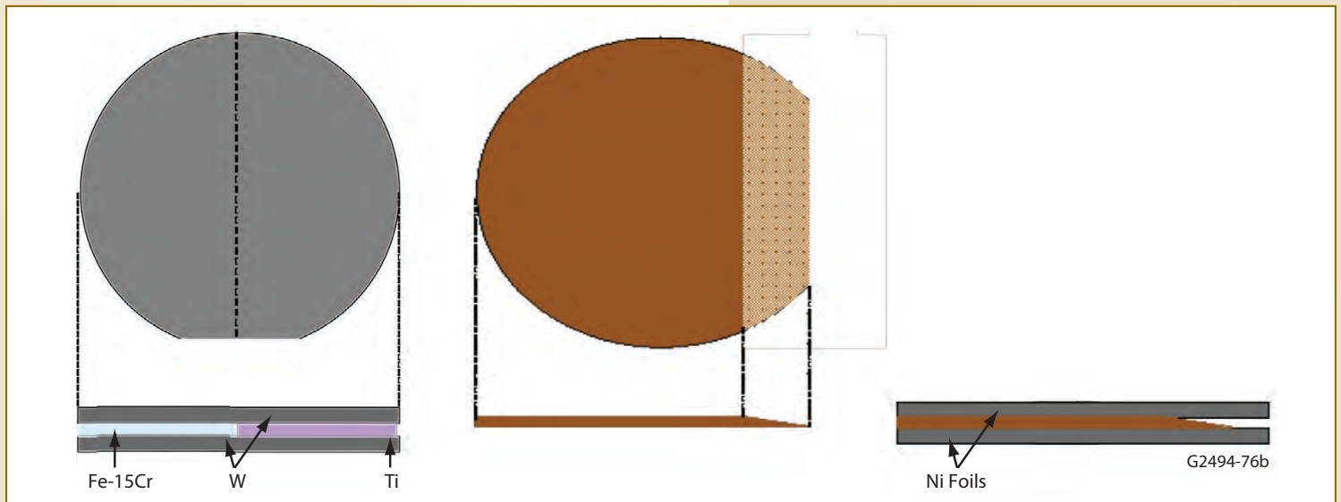
Figure 2. Two sample configurations include: (left) a typical diffusion multiple specimen for Fe-W-Cr-Ti and (right) a nickel foil wedge specimen stack-up for in situ helium implantation studies.
