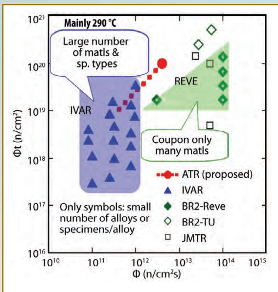
Figure 1. Flux-fluence map for reactor pressure vessel steel irradiations.
