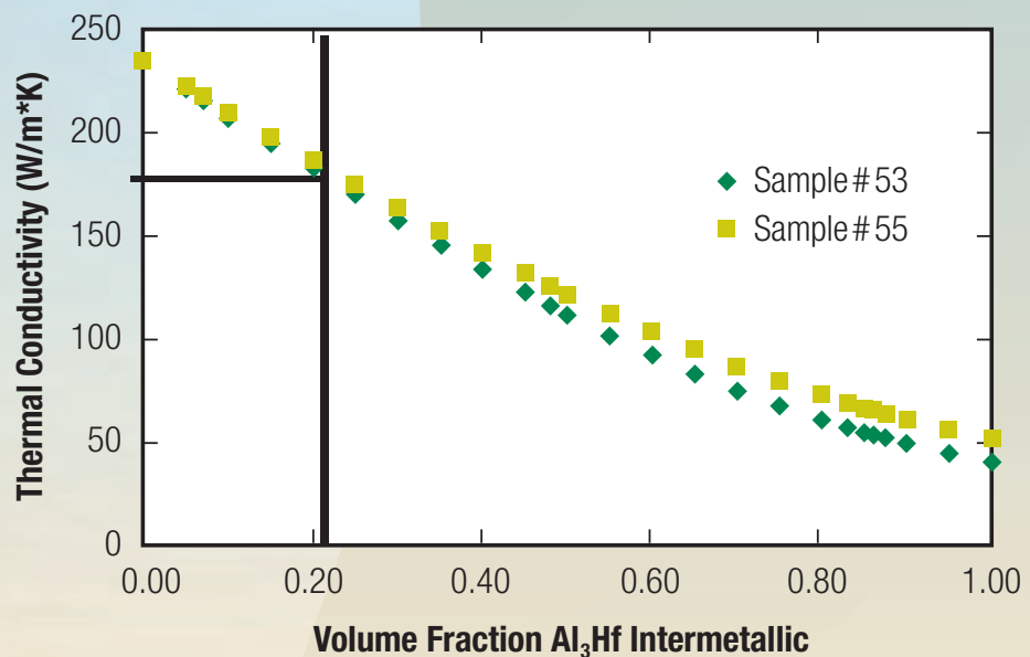
Figure 1. The graph shows the thermal conductivity for two samples of Al_3Hf in an Al matrix at different volume fractions: sample #55 ( Al_3Zr type) with predominantly high-temperature phase and sample #53 ( Al_3Ti type) with low-temperature phase.
